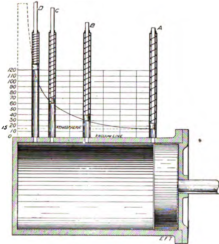
FIG. 227. —Diagrammatic Section of a Cylinder illustrating the compression and expansion of gases. This cylinder is filled with air at atmospheric pressure which represents a uniform 14.7 pounds to the square inch behind the piston, as shown by the position of the piston in the small cylinder, A . When the piston of the large cylinder is moved through half the length of the stroke, it shows 30 pounds pressure, as shown by the position of the piston in small cylinder, B ; when at three-quarters stroke, 60 pounds, as shown by position of the piston, C ; when at seven-eighths stroke, 120 pounds, as shown by position of piston, D . At full stroke it would be 240 pounds, the diagram behind the small piston giving the compression curve from 15 to 240.
